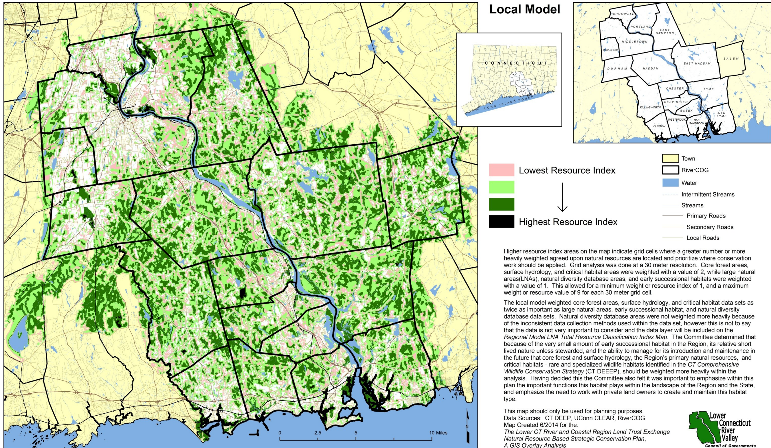
Figure 1 – Local Model.
